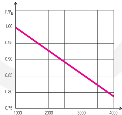
Power reduction at less cooling
